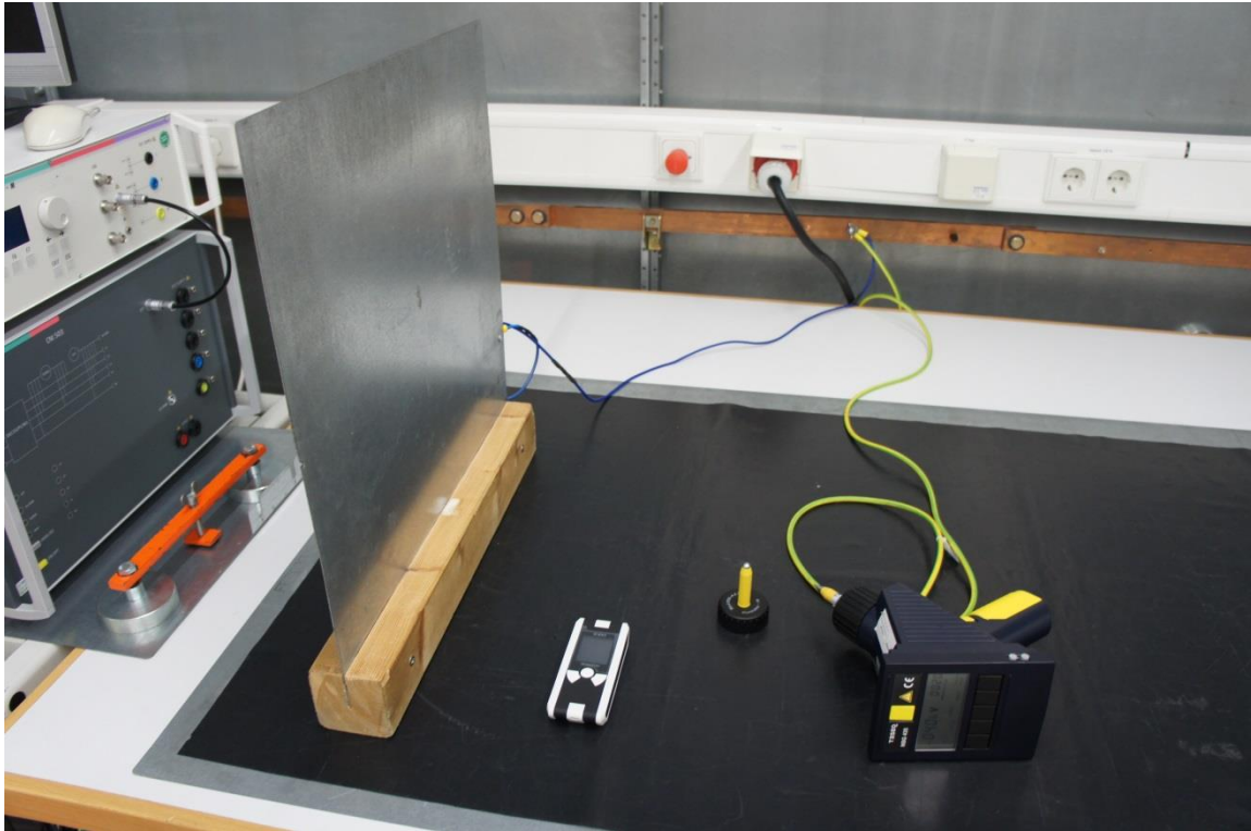
Picture 5: Test setup ESD
